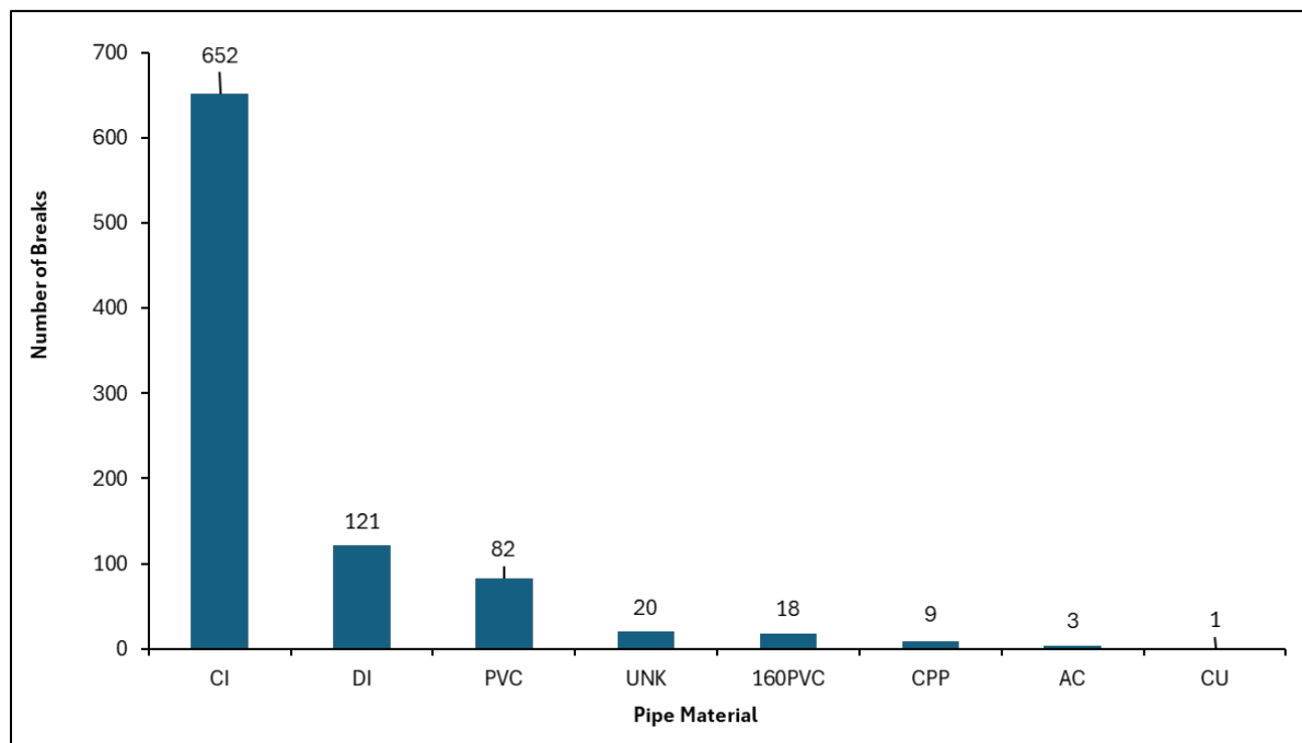
Figure 9: Number of Breaks by Pipe Material
